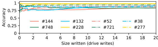
Fig. 7. Page Classifier prediction accuracy over time (cumulative).
