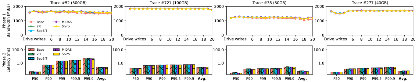
Fig. 11. I/O bandwidth and latency on low-WA traces.
