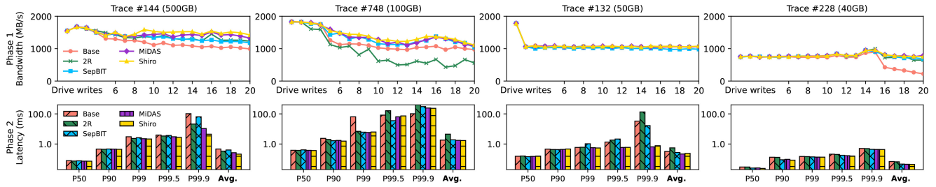
Fig. 10. I/O bandwidth and latency on high-WA traces.
