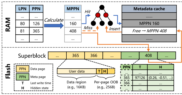
Fig. 5. Flash data layout and RAM metadata cache management.
