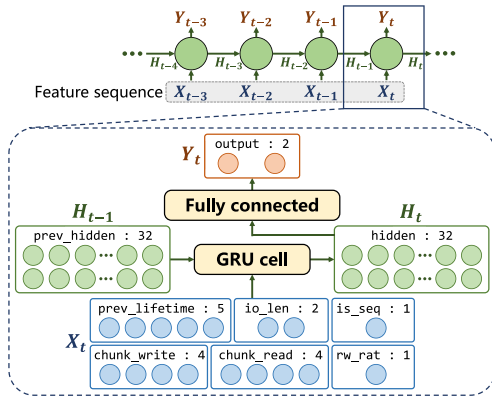
Fig. 4. Structure of the Page Classifier model.
