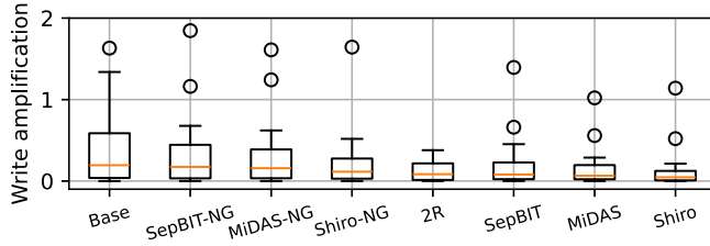
Fig. 8. WA on Alibaba Cloud traces with GC/user data separation disabled.
