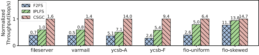
Fig. 4. Performance overview.
