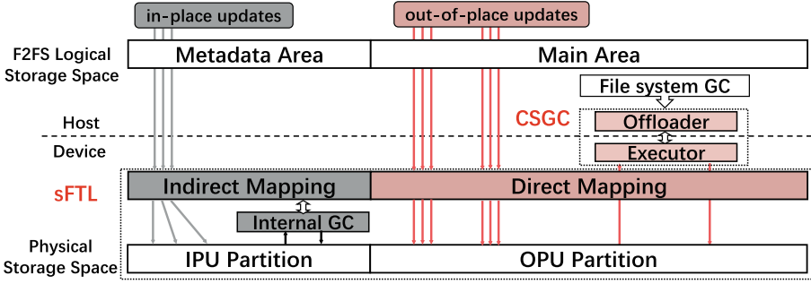
Fig. 3. Decoupled storage management through sFTL.
