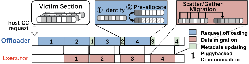
Fig. 2. GC execution pipeline.
